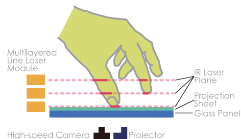
Figure 2: System architecture.
